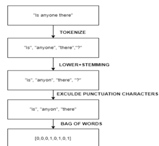
Figure 3 NLP Pre-Processing Pipeline
