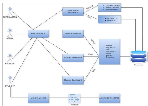
Figure 1 System Architecture of an E-Learning Management System
